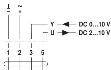
SH24A-MF..
